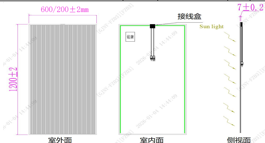
Figure 1: Three-view component
